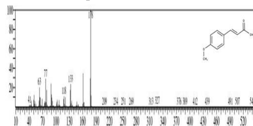
Figure 3. Mass Spectra of APMS Compounds
