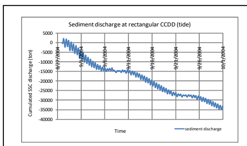
Gambar 11. Sedimen transport kumulatif CCDD akibat arus
