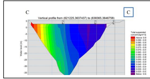
Gambar 6. Penampang CC saat spring-
