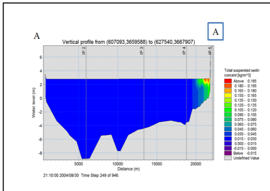
Gambar 4. Penampang AA saat spring-tide
