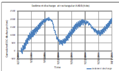
Gambar 9. Sedimen transport kumulatif AABB akibat arus
