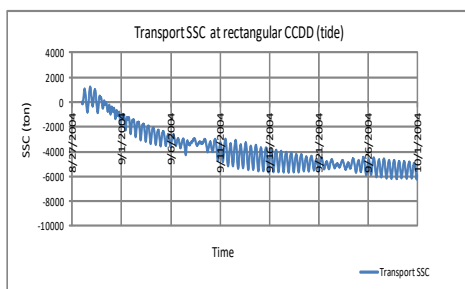
Gambar 10. Trend transport sedimen area CCDD akibat arus
