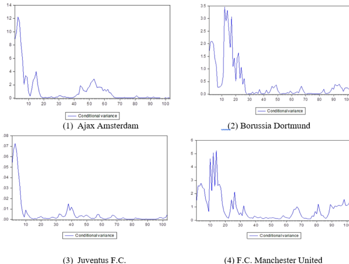
Figure 2. Conditional Variance
