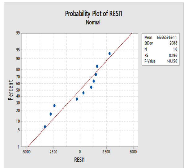
Gambar 1. Plot Normalitas
