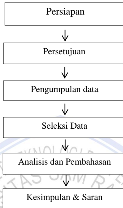
Gambar 2. Prosedur Penelitian
