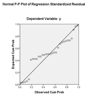
Gambar 2. Normal P-Plot of Regression Standarized Residual
