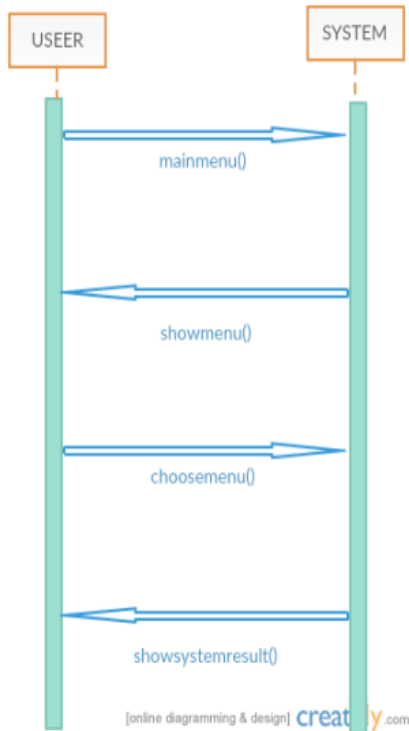
Gambar 5. Sequence Diagram
