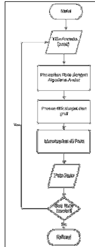
Gambar 10. Flowchart System
