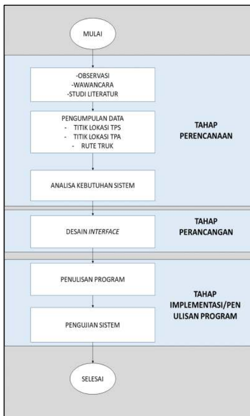
Gambar 4. Prosedur Penelitian
