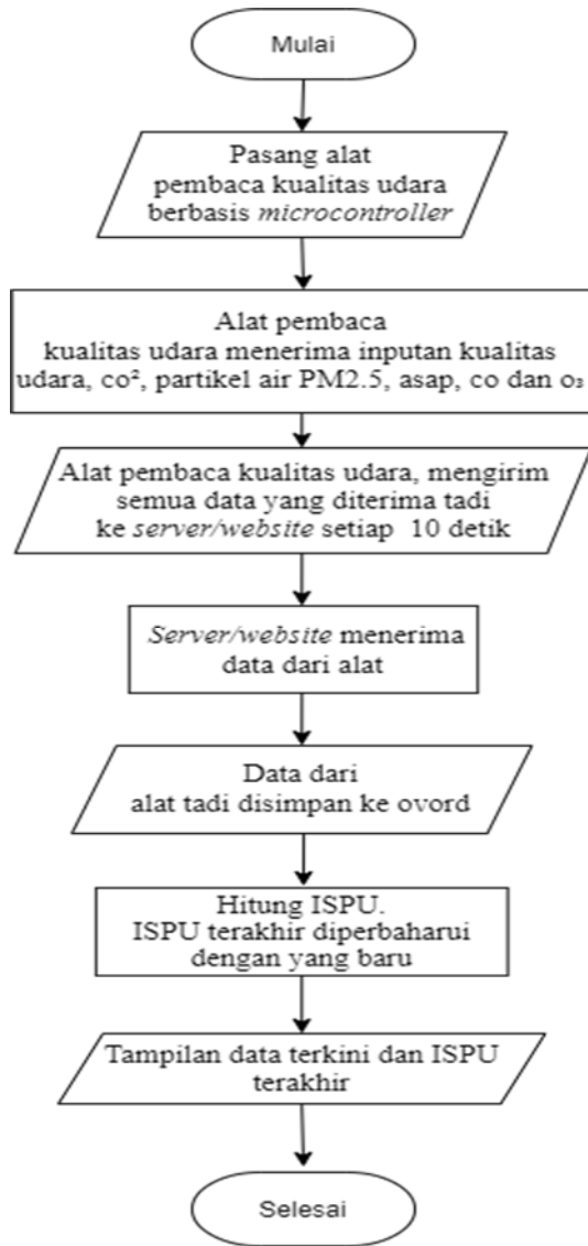
Gambar 11. Flowchart system
