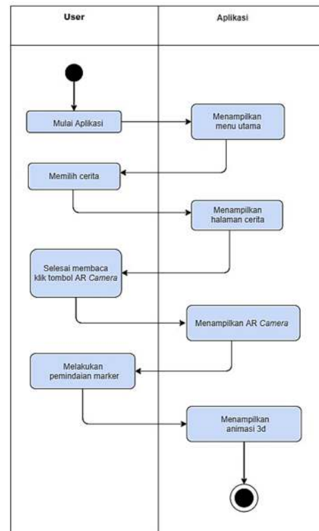
Gambar 4. Activity Diagram Menu Utama
