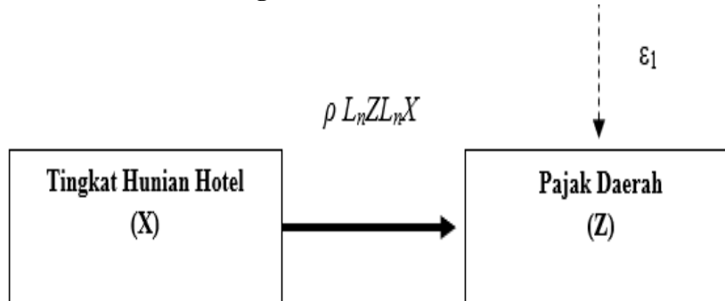
Gambar 3. Diagram Jalur Model Sub-Struktural 1
