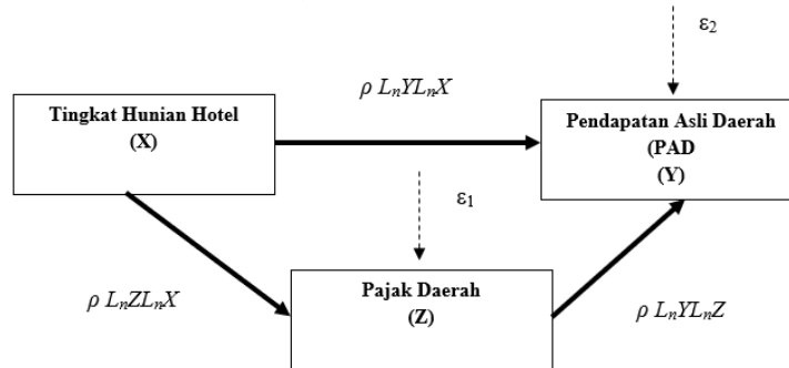
Gambar 2. Diagram Jalur Model Struktural
