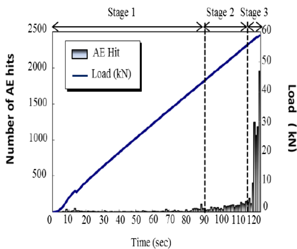
(a)SFRC Specimen
