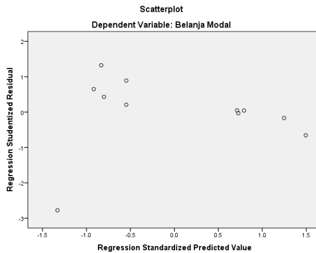
Gambar 2 Diagram scatterplot
