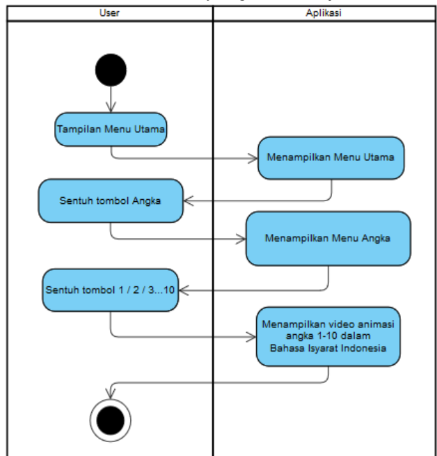
Gambar 5. Activity Diagram Angka
