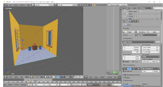
Gambar 9. Modeling Ruang
