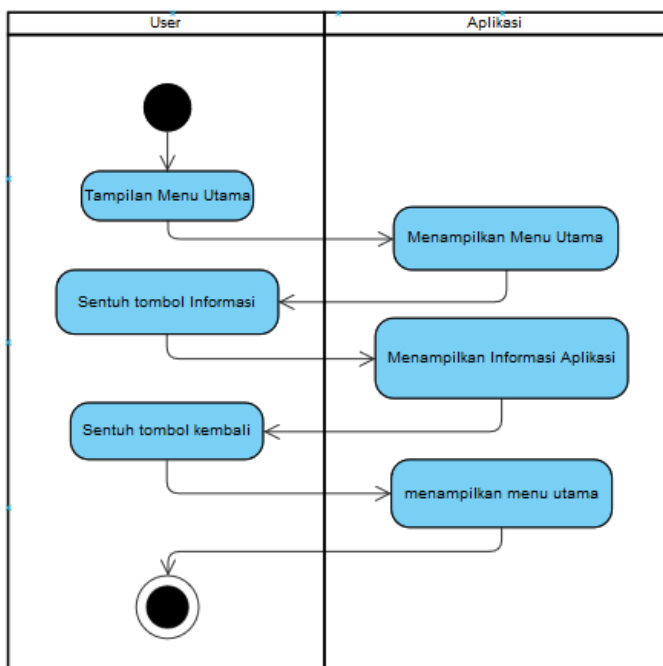
Gambar 6. Activity Diagram Menu Informasi
