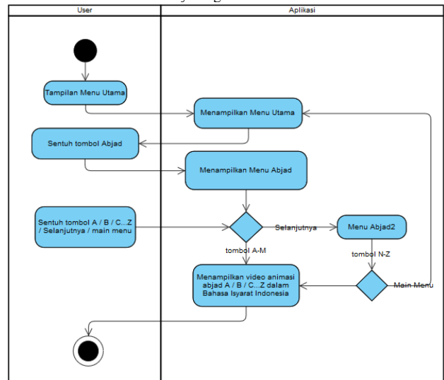
Gambar 4. Activity Diagram Menu Abjad
