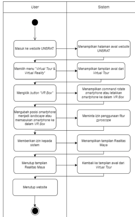
Gambar 5. Activity Diagram Realitas Maya
