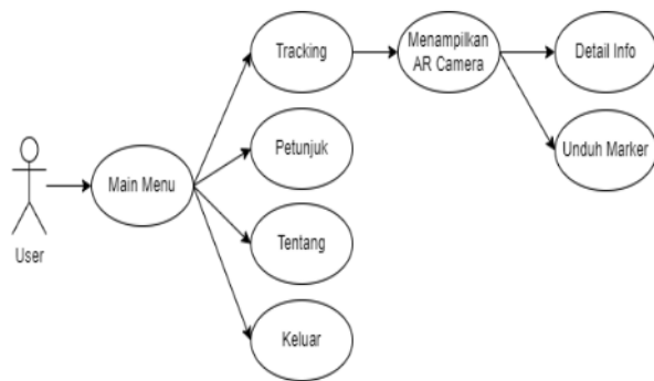
Gambar 3. Use case
