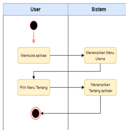
Gambar 7. Activity Diagram Tentang
