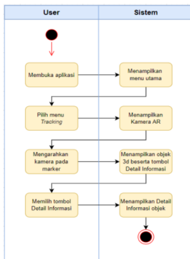
Gambar 5. Activity Diagram Main Menu
