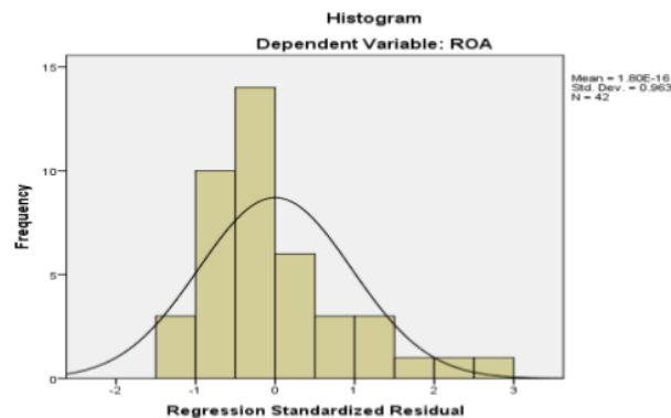
Gambar 1. Gambar Histogram
