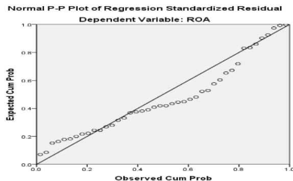
Gambar 2. Normal Probabilityplot
