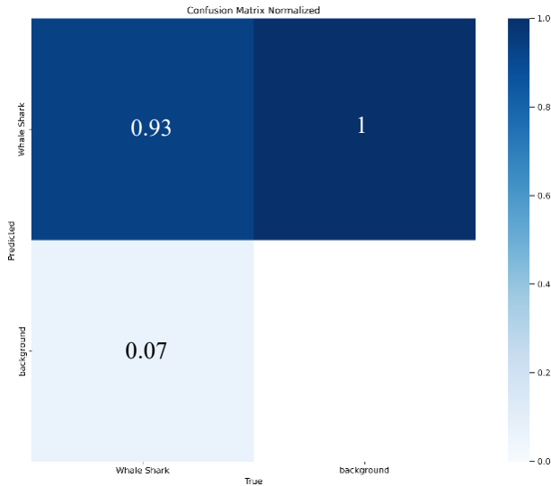
Fig. 3. Confusion Matrix Normalized.
