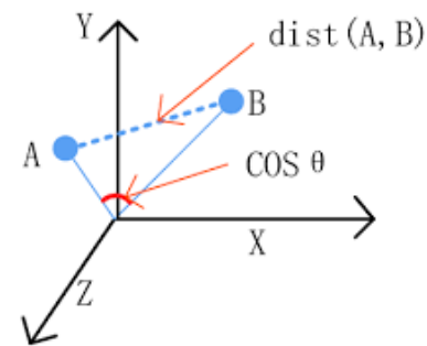
Gambar 4. Cosine Similarity
