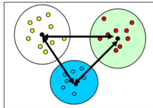
Gambar 3. Clustering K-Means
