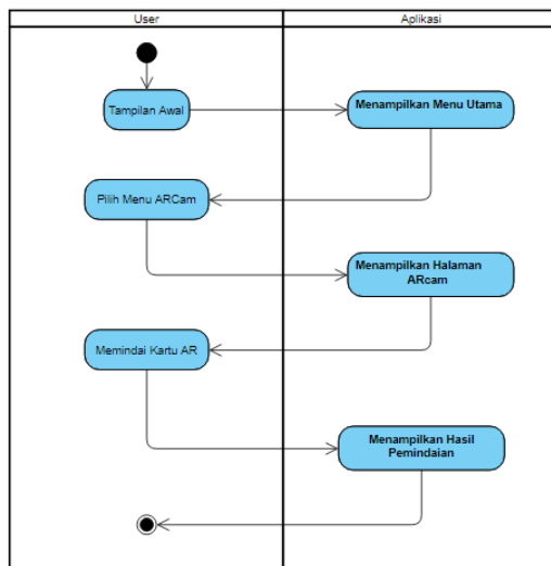
Gambar 4. Activity Diagram Menu Utama
