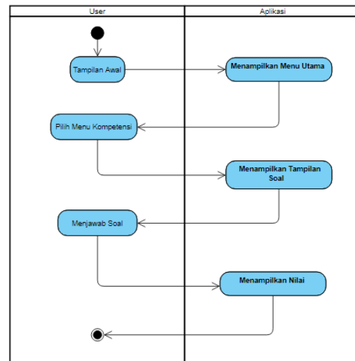
Gambar 6. Activity Diagram Menu Kompetensi
