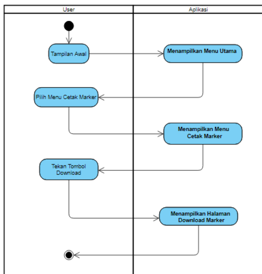
Gambar 8. Activity Diagram Menu Cetak Marker
