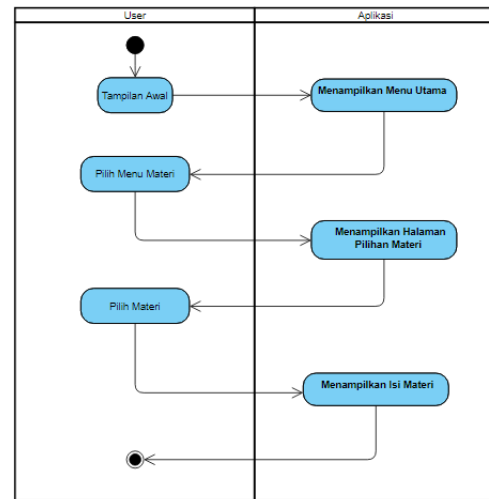
Gambar 5. Activity Diagram Menu Materi
