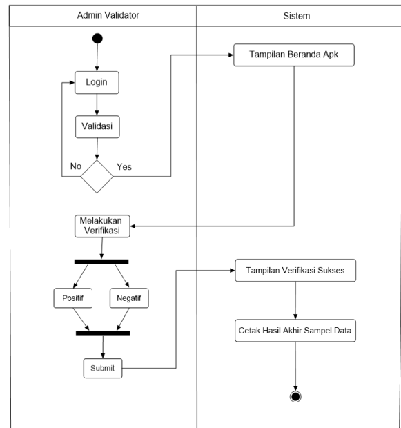
Gambar 3. Activity diagram validator
