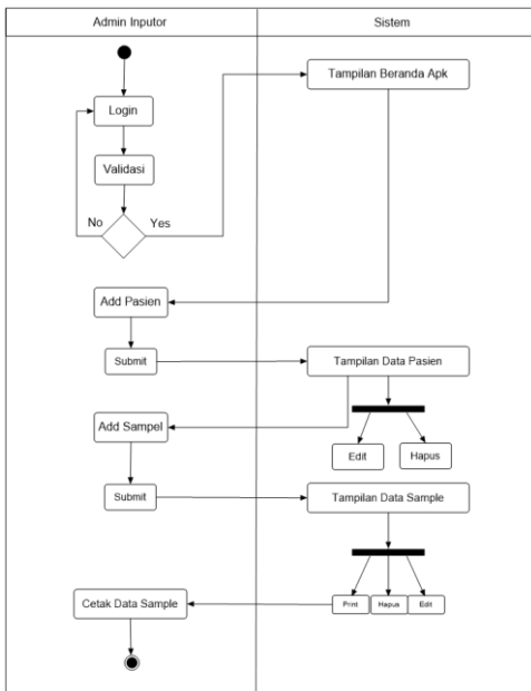
Gambar 1. Activity diagram inputor
