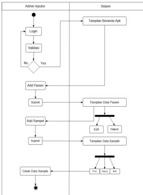
Gambar 2. Activity diagram inputor
