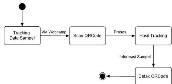
Gambar 5. State diagram tracking data sampel covid-1
