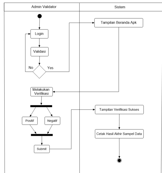
Gambar 4. Activity diagram validator
