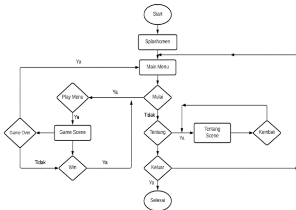
Gambar 3. Flowchart Game Solar System
