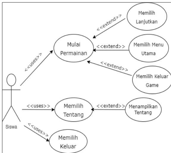
Gambar 2. User Case Diagram
