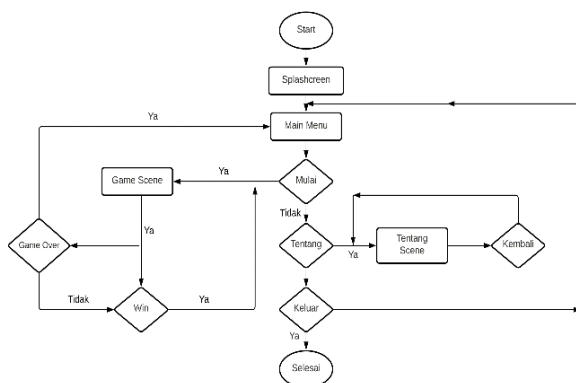
Gambar 3. Flowchart Game Solar System
