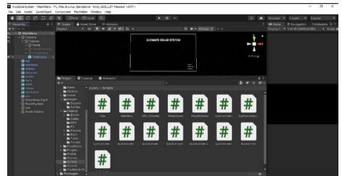
Gambar 22. Asset Script
