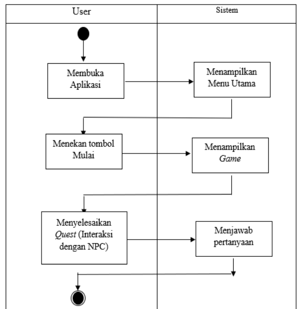
Gambar 4. Activity Diagram Mulai
