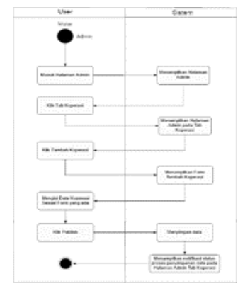
Gambar 7. Activity Diagram menambah data Koperasi
