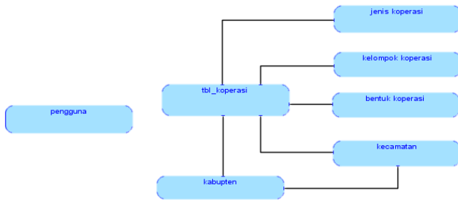
Gambar 3. Conceptual Entity Relationship Diagram
