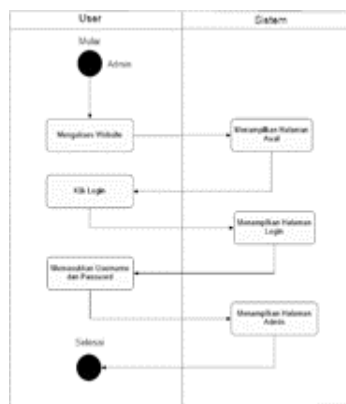
Gambar 6. Activity Diagram sisi Admin
