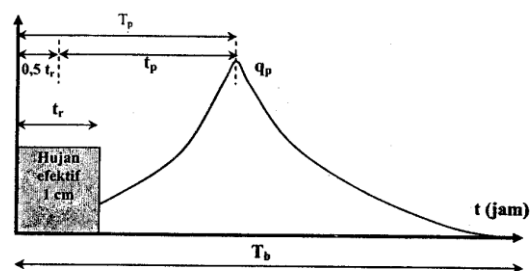
Gambar 2 : Skema Model HSS Snyder Standar (Tp= 5,5 tr) (Sumber : I Made Kamiana, 2011)
