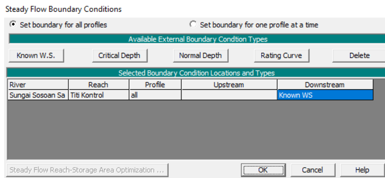
Gambar 13. Pengisian Reach Boundary Conditions
