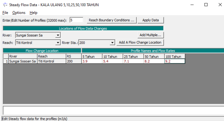
Gambar 12. Pengisian Data Debit
